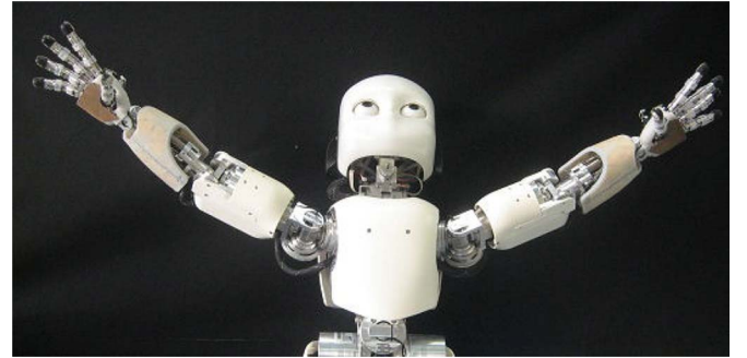
Fig. 7. iCub covered with artificial skin. Each arm has 384 sensing points: 23 PCBs in the forearm, four in the palm, and five in the fingertips, with 12 sensing points each. Note that the artificial skin requires few wires, which can all be routed inside the robot.
