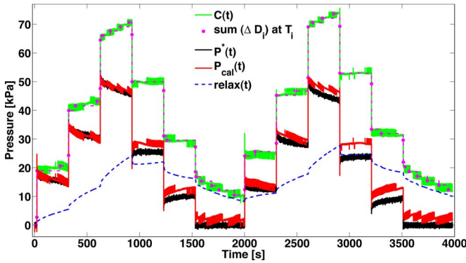
Fig. 18. Compensation of the relaxation of the silicone foam. We applied multistep, cyclic loading. C(t) is the uncorrected sensor measurements, \Delta D_i is stepwise approximation, \text{relax}(t) is the correction term, and P_{\text{cal}}(t) are the corrected measurements: P_{\text{cal}}(t) = C(t) - \text{relax}(t) . P^*(t) is the pressure calculated from the load cell, and there is a clear correspondence to P_{\text{cal}}(t) .
