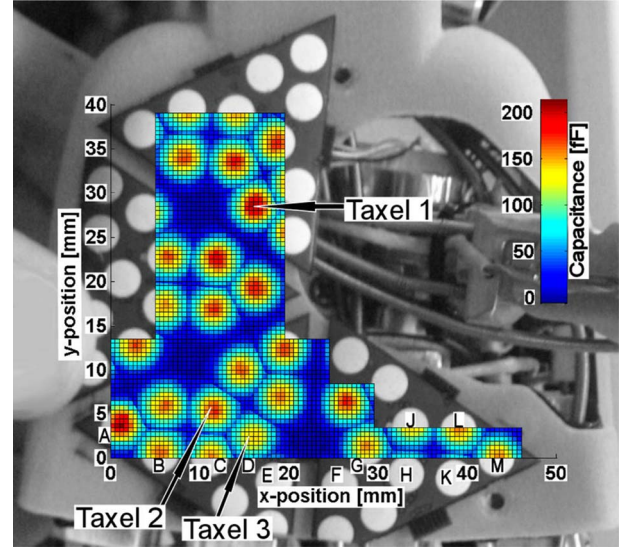
Fig. 11. Sensor response at different positions. We show the superimposed response of all taxels to a certain pressure (i.e., 150–160 kPa). In the background, we show a grayscale picture of the palm (without the silicone foam and the top conductive layer) to demonstrate the correspondence of the sensitive areas to the round pads on the PCBs. For the illustration, an old version of the PCBs is used, which better highlights the electrode areas.
